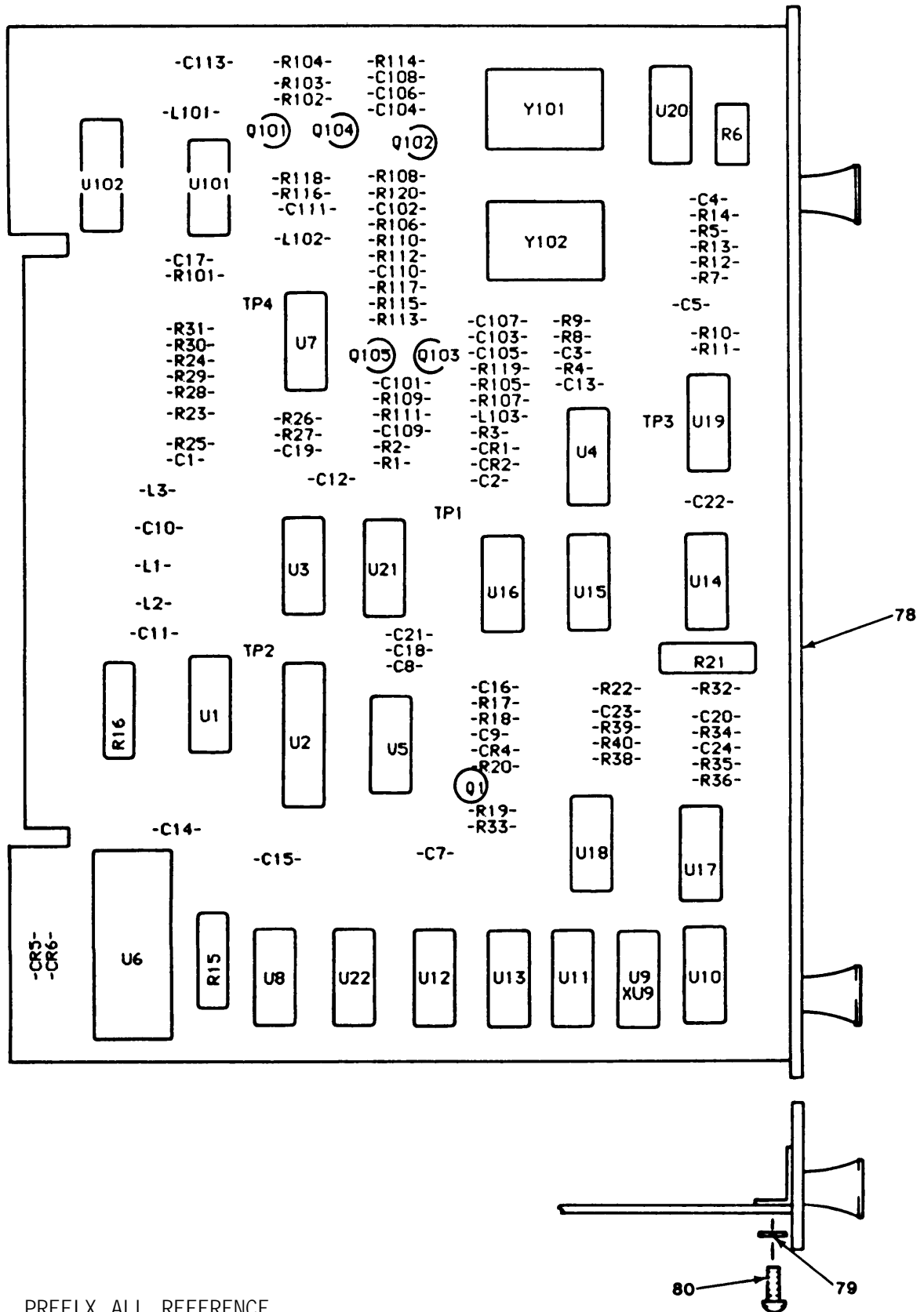
Figure 12. Analog to Digital Converter Circuit Card Assembly (Sheet 1 of 2).
